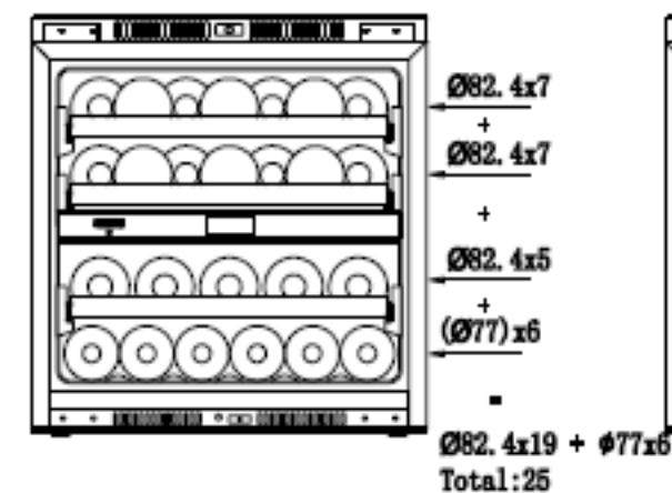
Bottle loading proposal#2 The shelf design is the same as proposal#1
